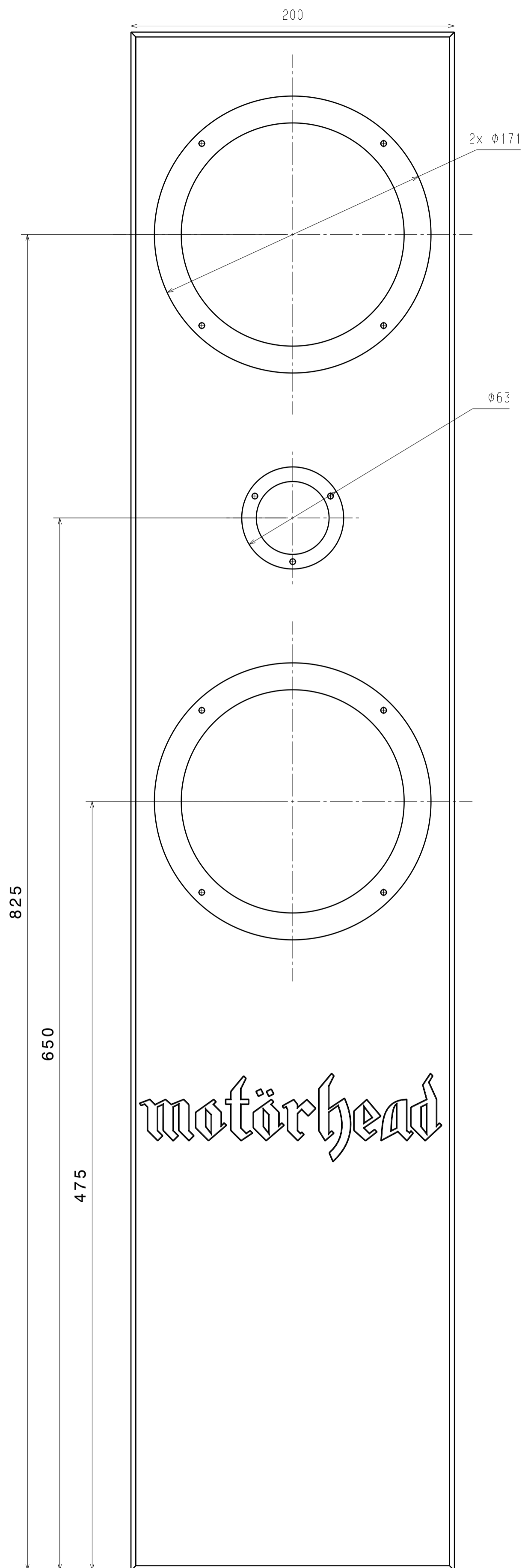
Front view Scale: 1:2
